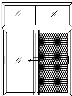
3-TRACK, 3-SHUTTER WITH MESH & TOP FIXED
