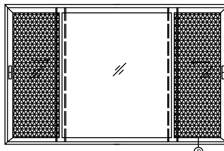
2-TRACK, 5-SHUTTER MIDDLE FIX WITH MESH
