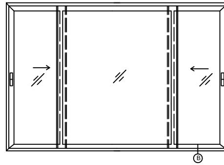
2-TRACK, 3-SHUTTER MIDDLE FIX
